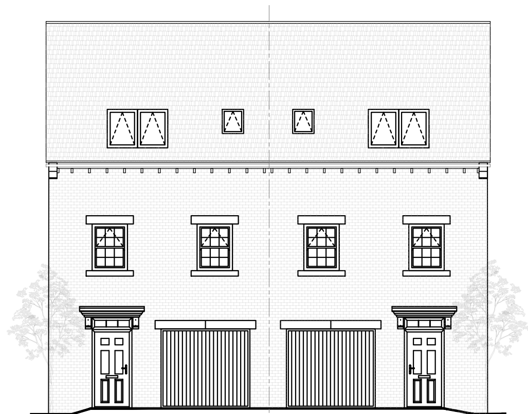
FRONT ELEVATION
