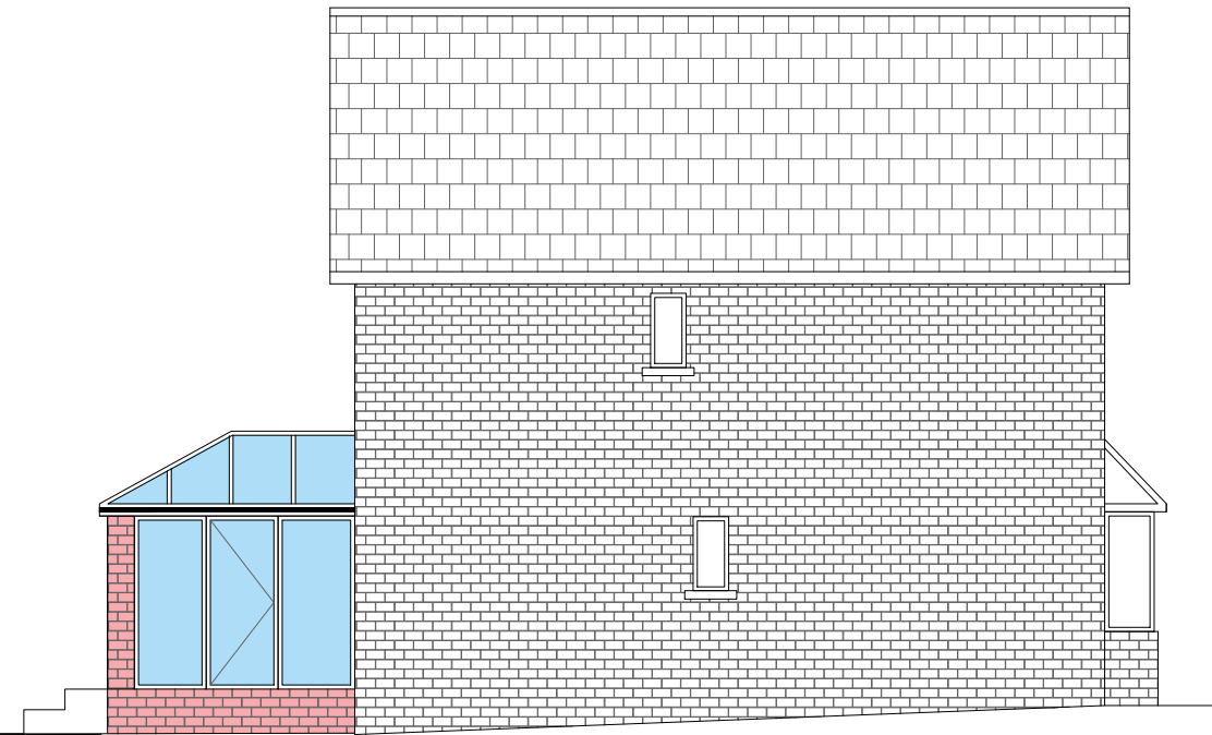
PROPOSED REAR ELEVATION (North)
