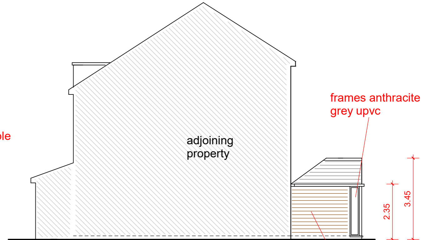
right side (southeast) elevation
