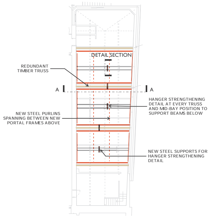
PLAN VIEW OF ROOF STRUCTURE NTS
