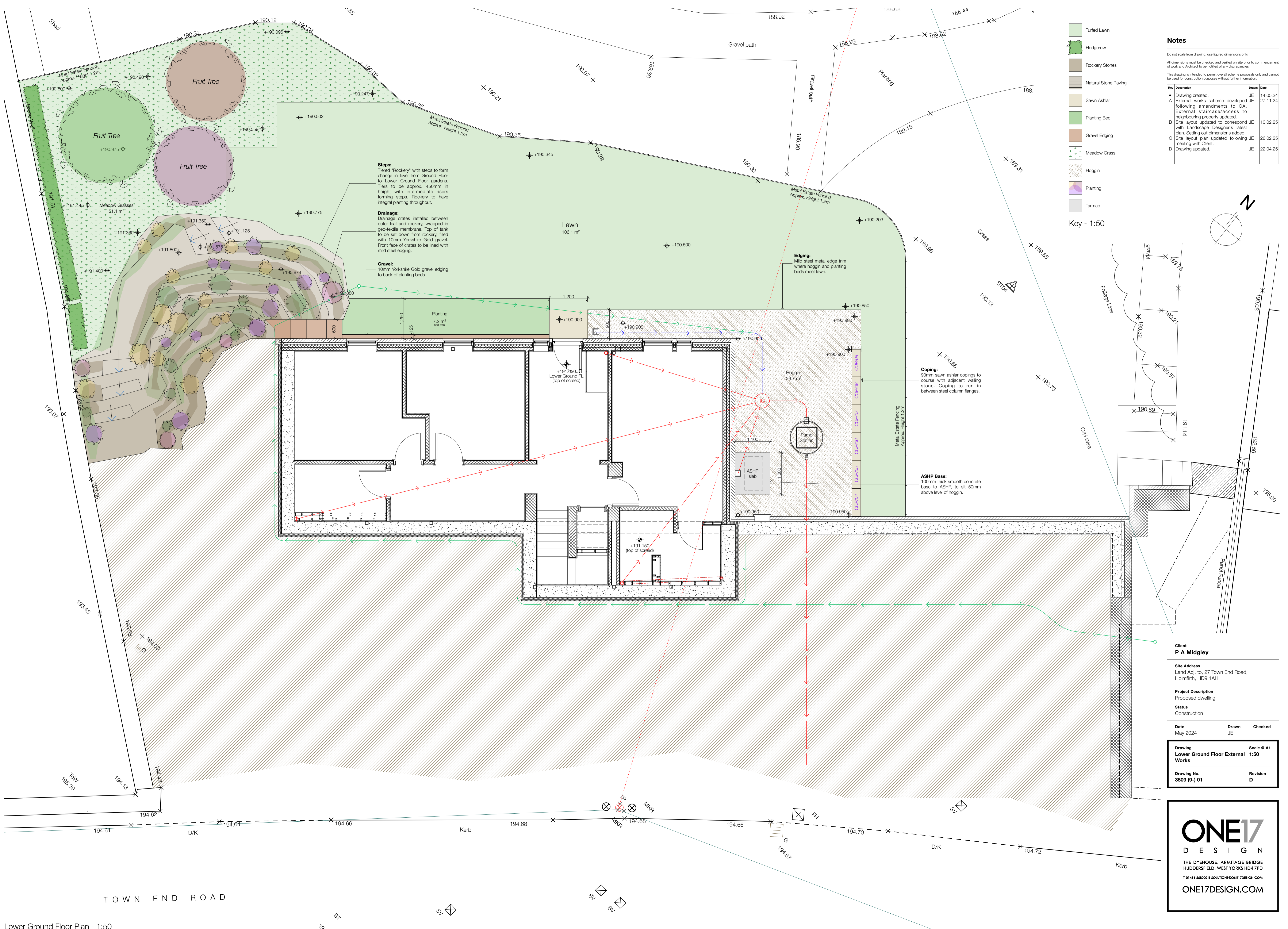
Lower Ground Floor Plan - 1:50
