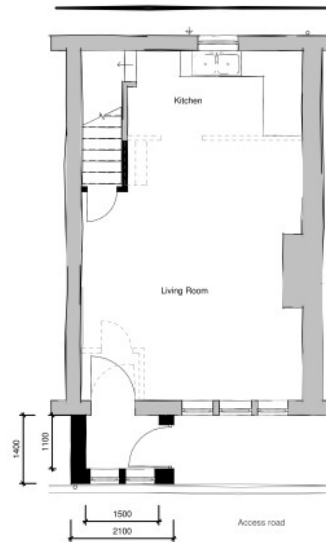
Ground Floor 1 : 50
