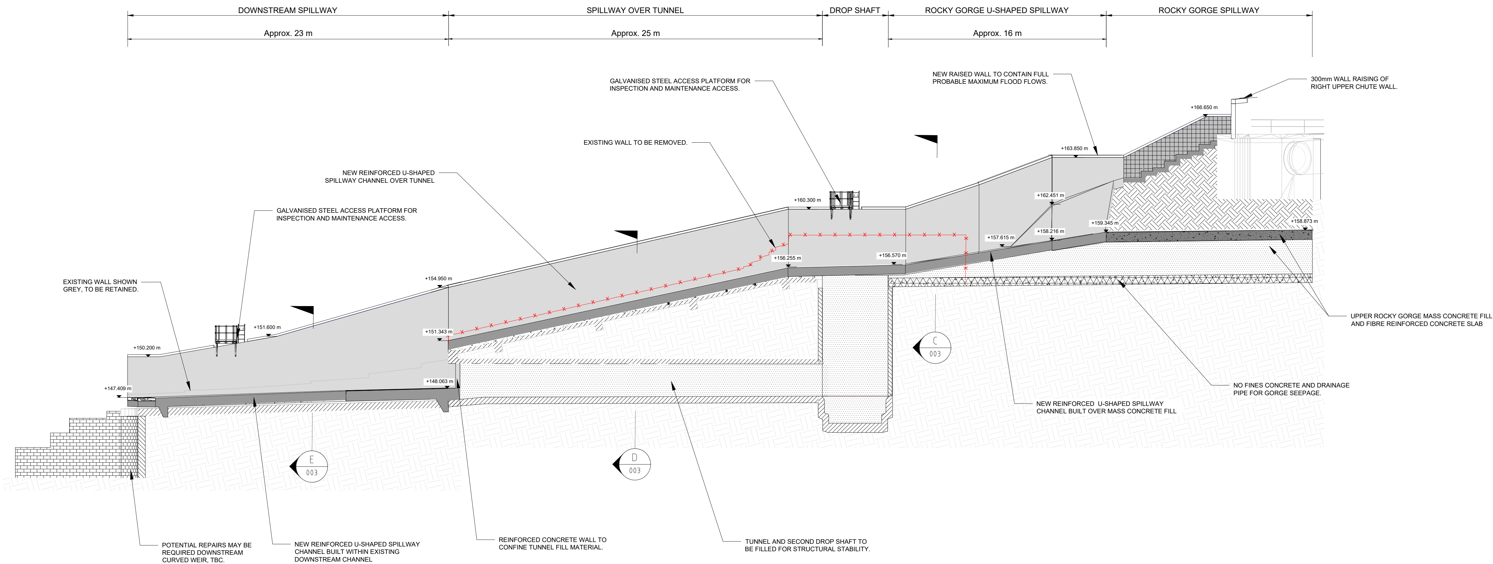
SPILLWAY LONG SECTION - A - A' REFER DRAWING 001 N.T.S.
