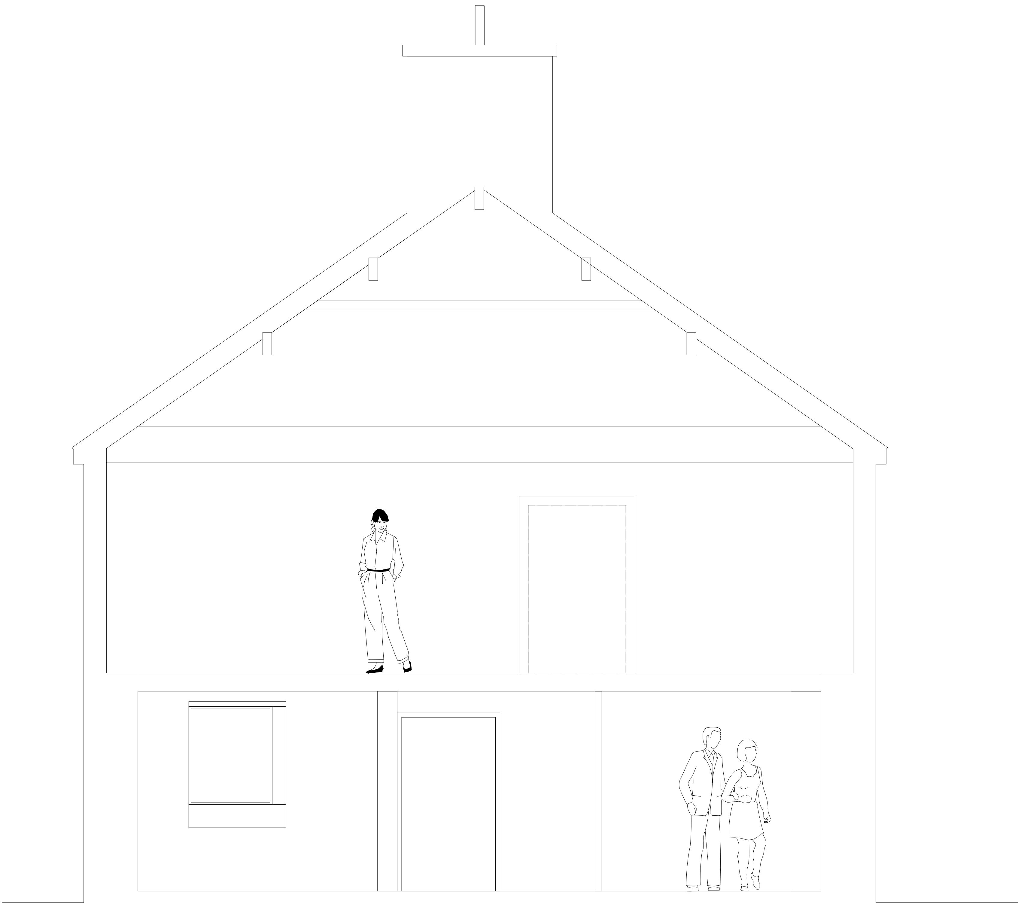
Section BB
