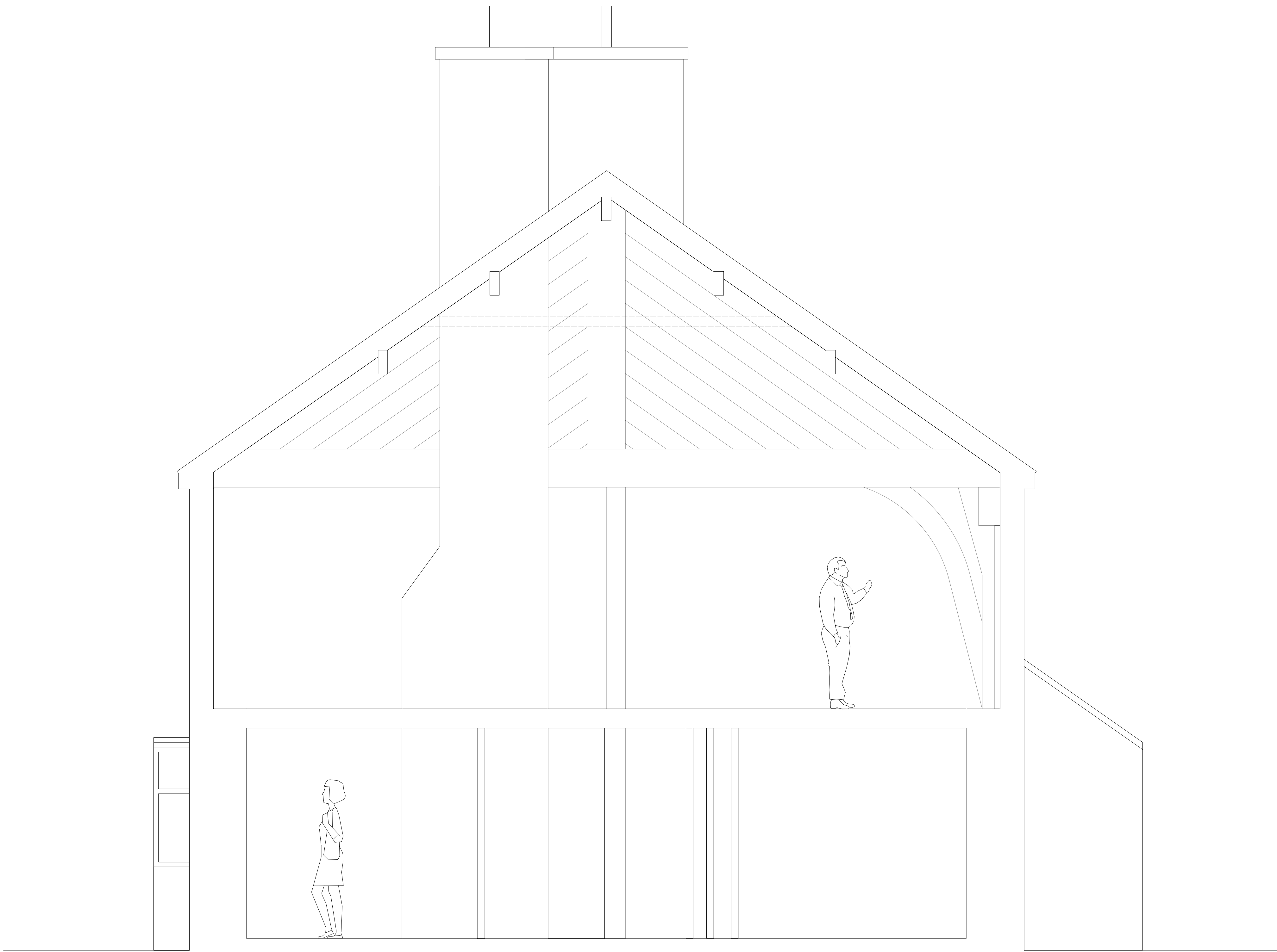
Section AA
