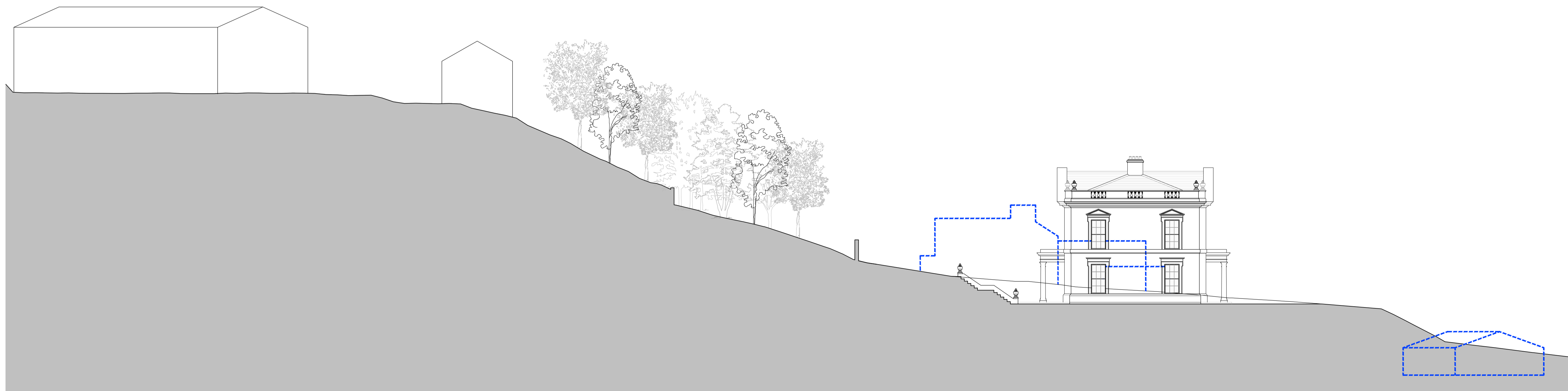
WEST SECTIONAL ELEVATION AS PROPOSED
