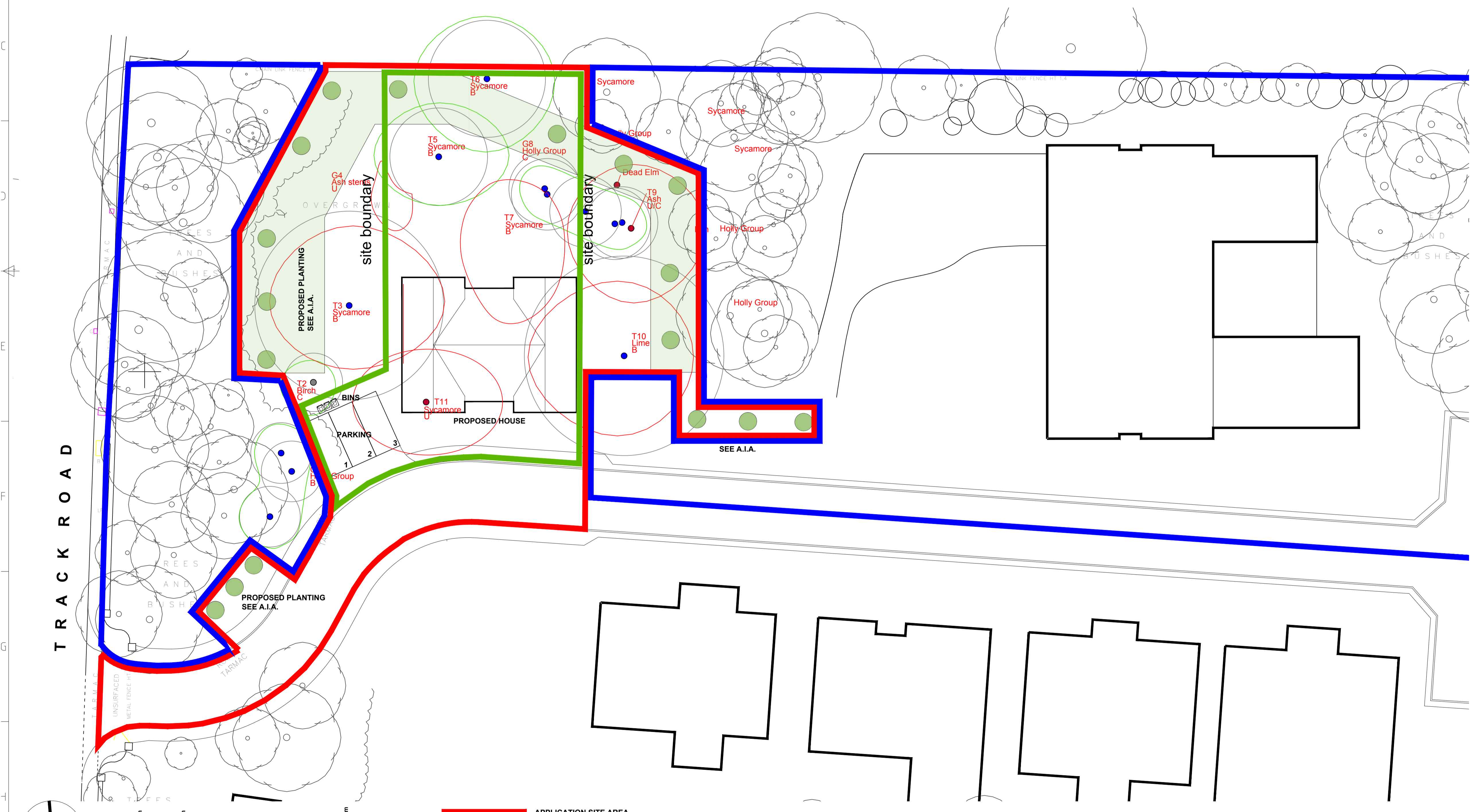
SITE PLAN AND ROOF PLAN AS PROPOSED
