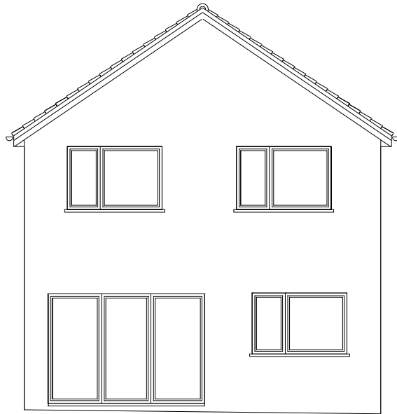
REAR - EXISTING ELEVATION
