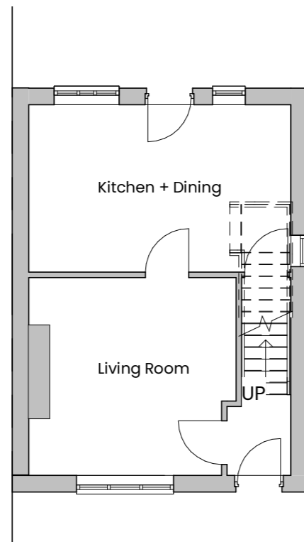
1 01. Ground Floor Plan 1:100
