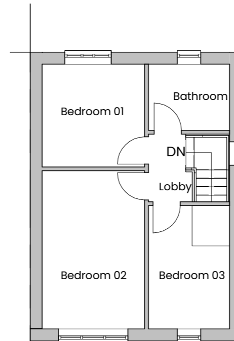
2 02. First Floor Plan 1:100
