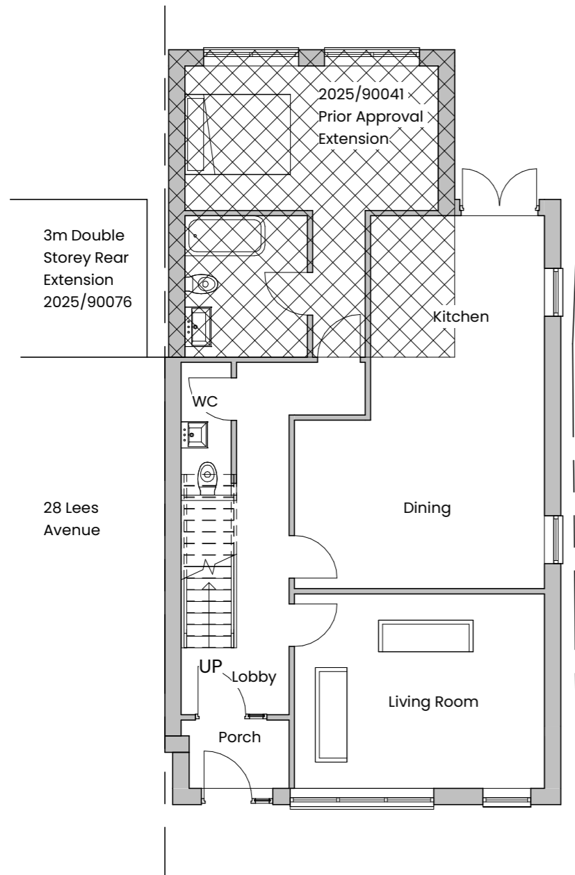
1 04. Proposed Ground Floor Plan 1:100
