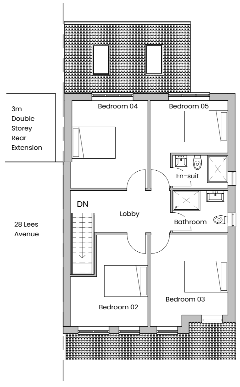
2 05. Proposed First Floor Plan 1:100
