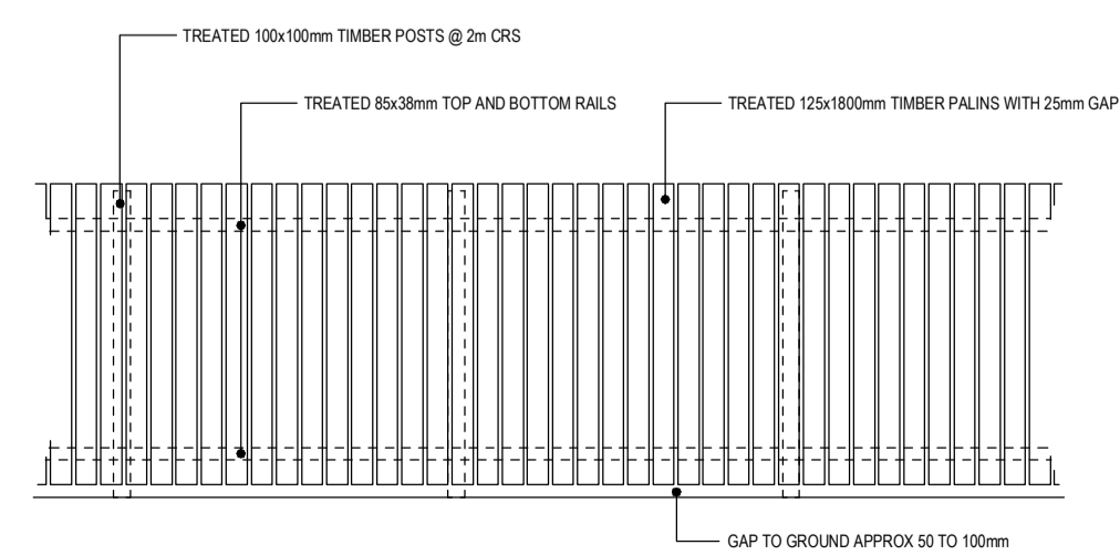
TYPICAL FENCING ELEVATION 1:50
