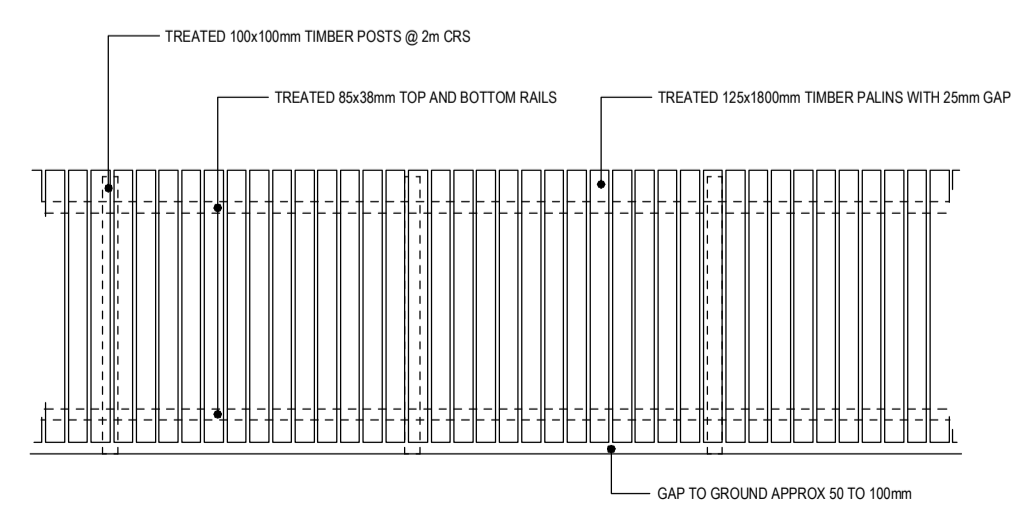
TYPICAL FENCING ELEVATION 1:50
