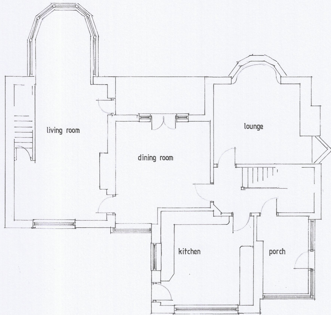
EXISTING PLAN
