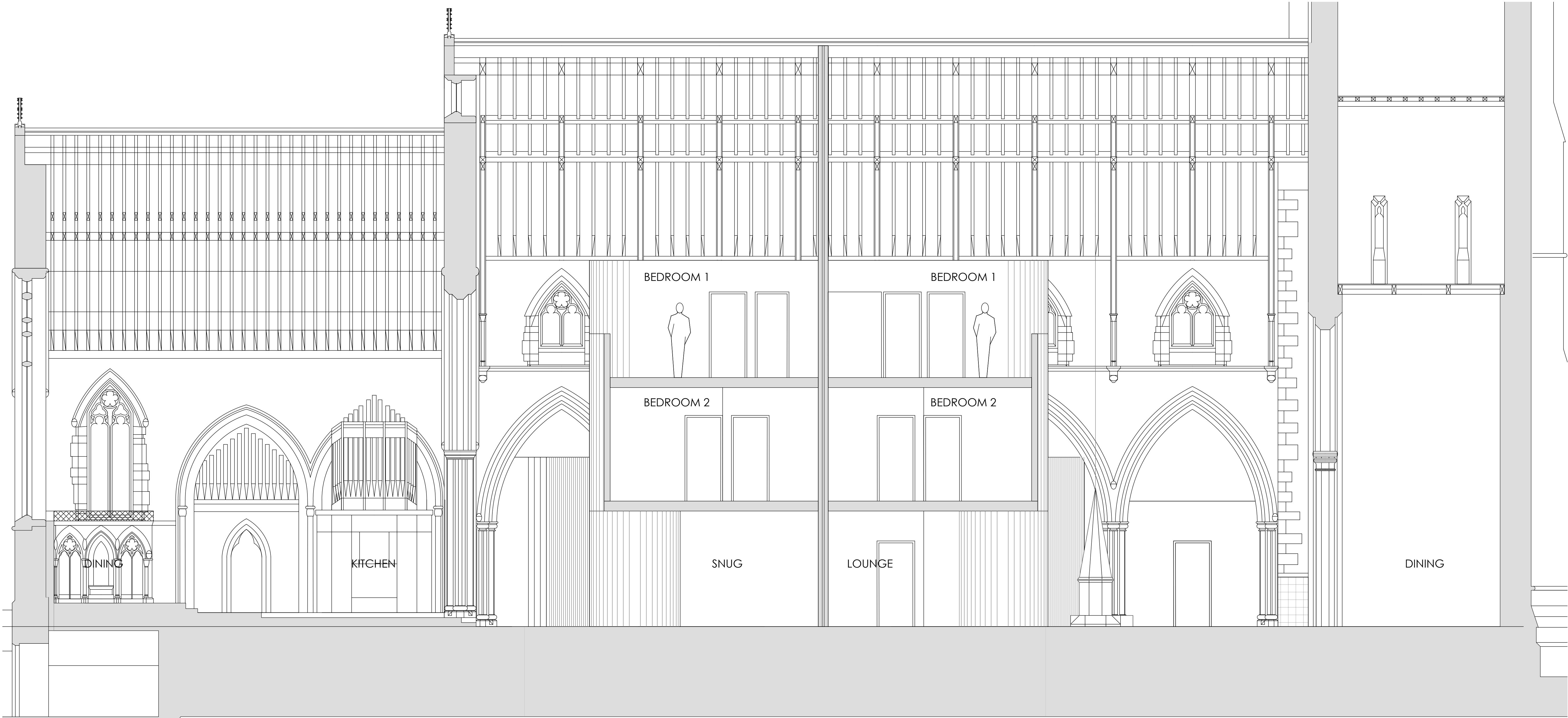
PROPOSED SECTION B-B - MAIN HALL SCALE 1:50
