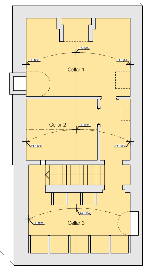
Existing Cellar Plan - 1:100
