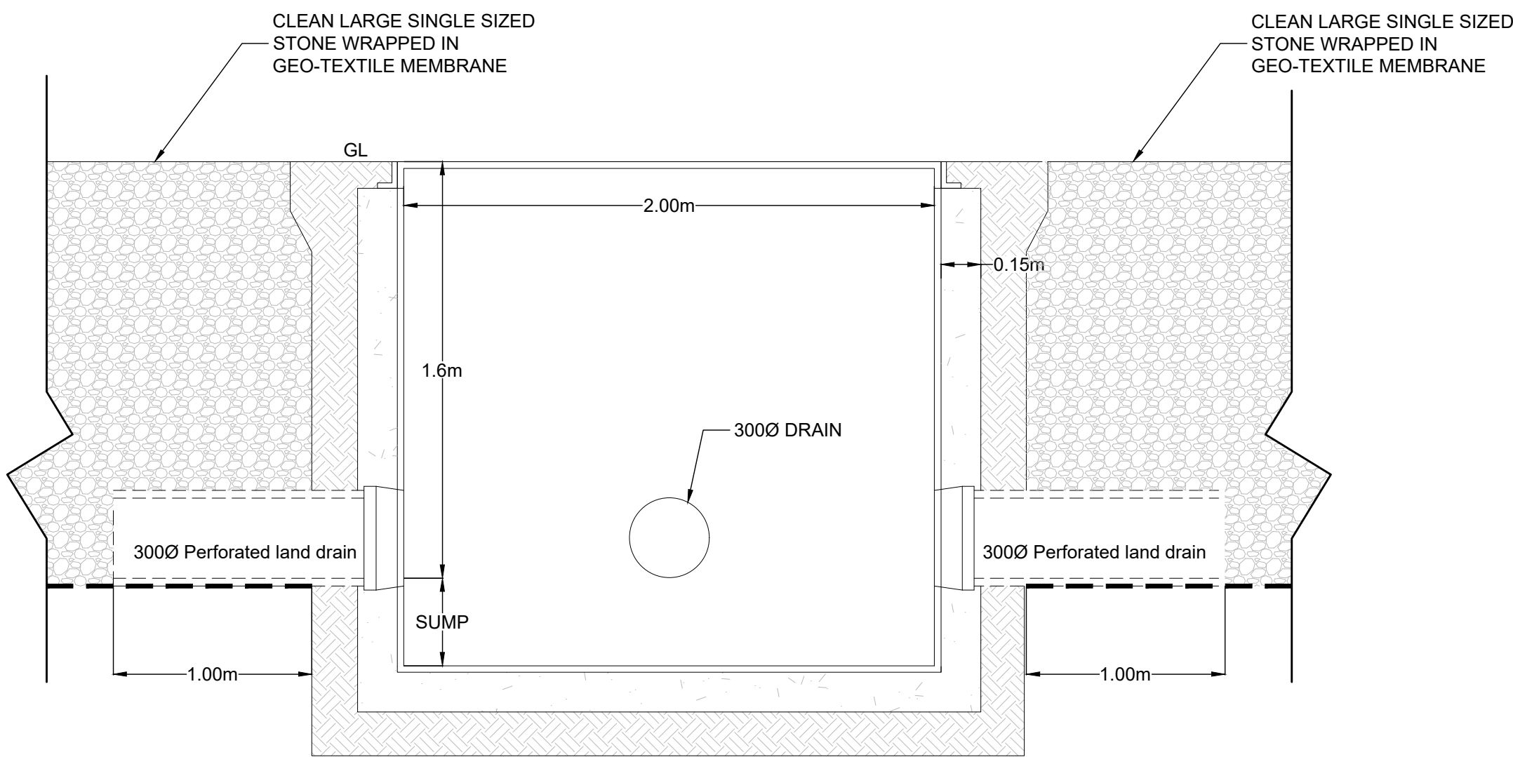
SURFACE WATER INFILTRATION TANK Scale 1:20
