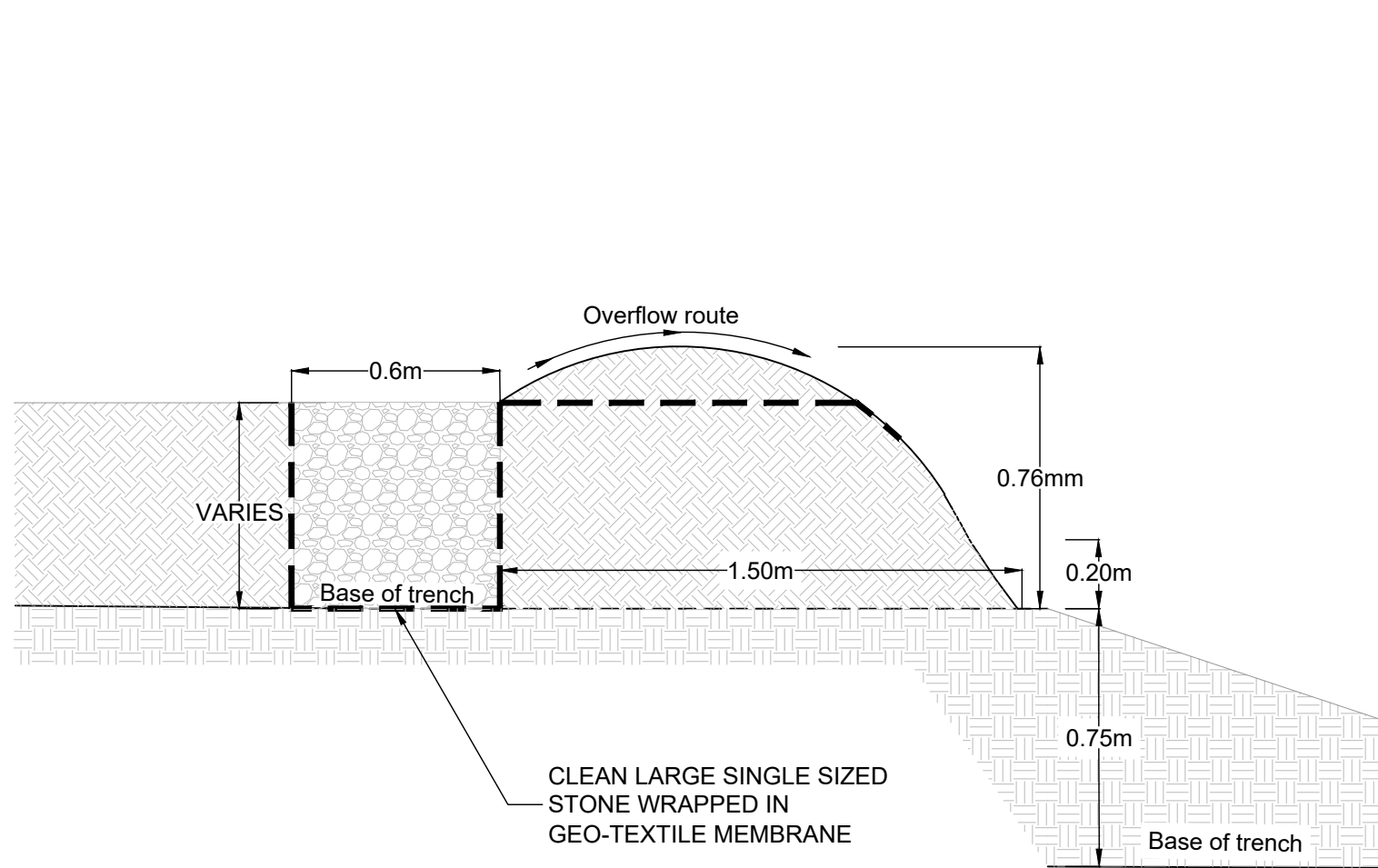
SECTION THROUGH PROPOSED SURFACE WATER LAND DRAIN Scale 1:20
