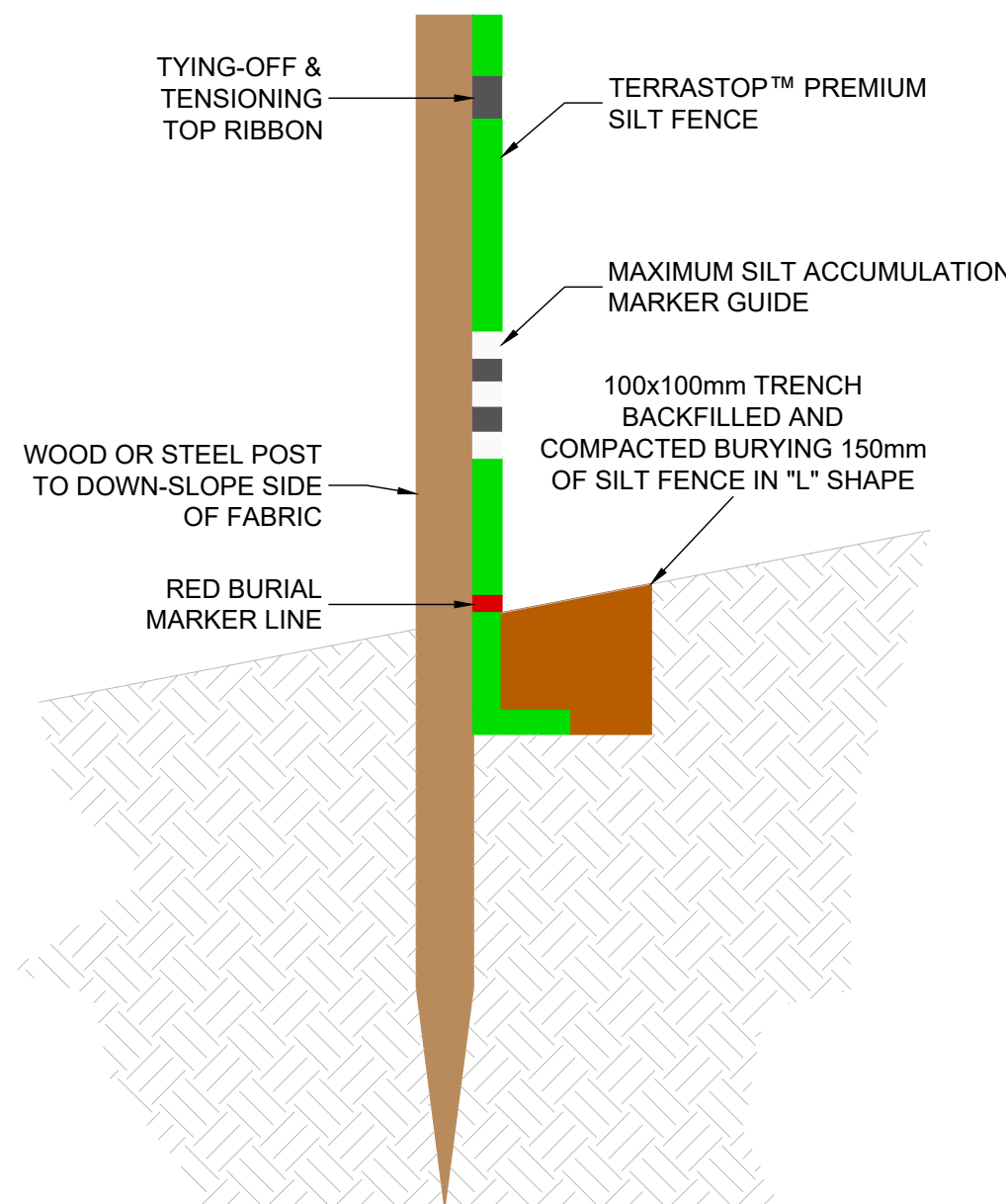
HY-TEX TERRASTOP PREMIUM SILT FENCE SECTION Not to Scale
