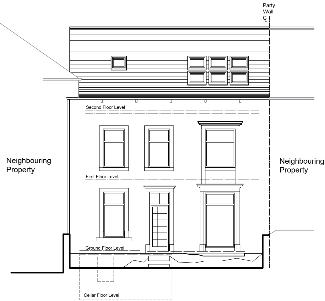
West Elevation (rear)
