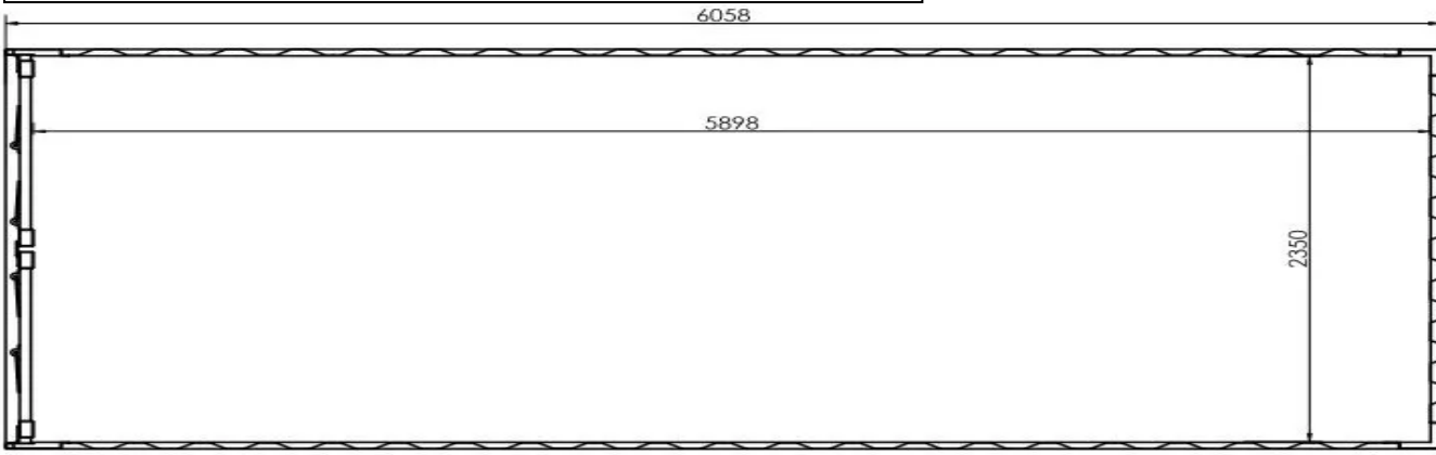
6.058M Shipping Container - Plan
