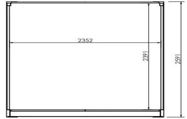
6.058M Shipping Container - Front Elevation
