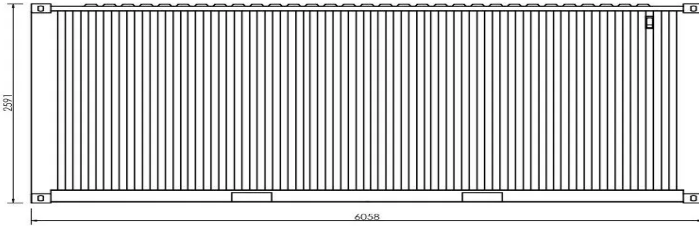
6.058M Shipping Container - Side Elevation
