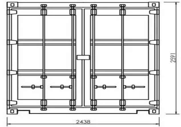
6.058M Shipping Container - Door Elevation
