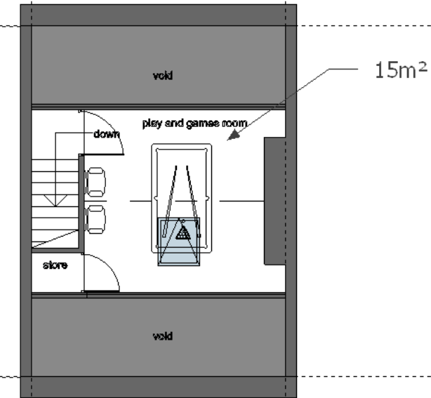
proposed attic
