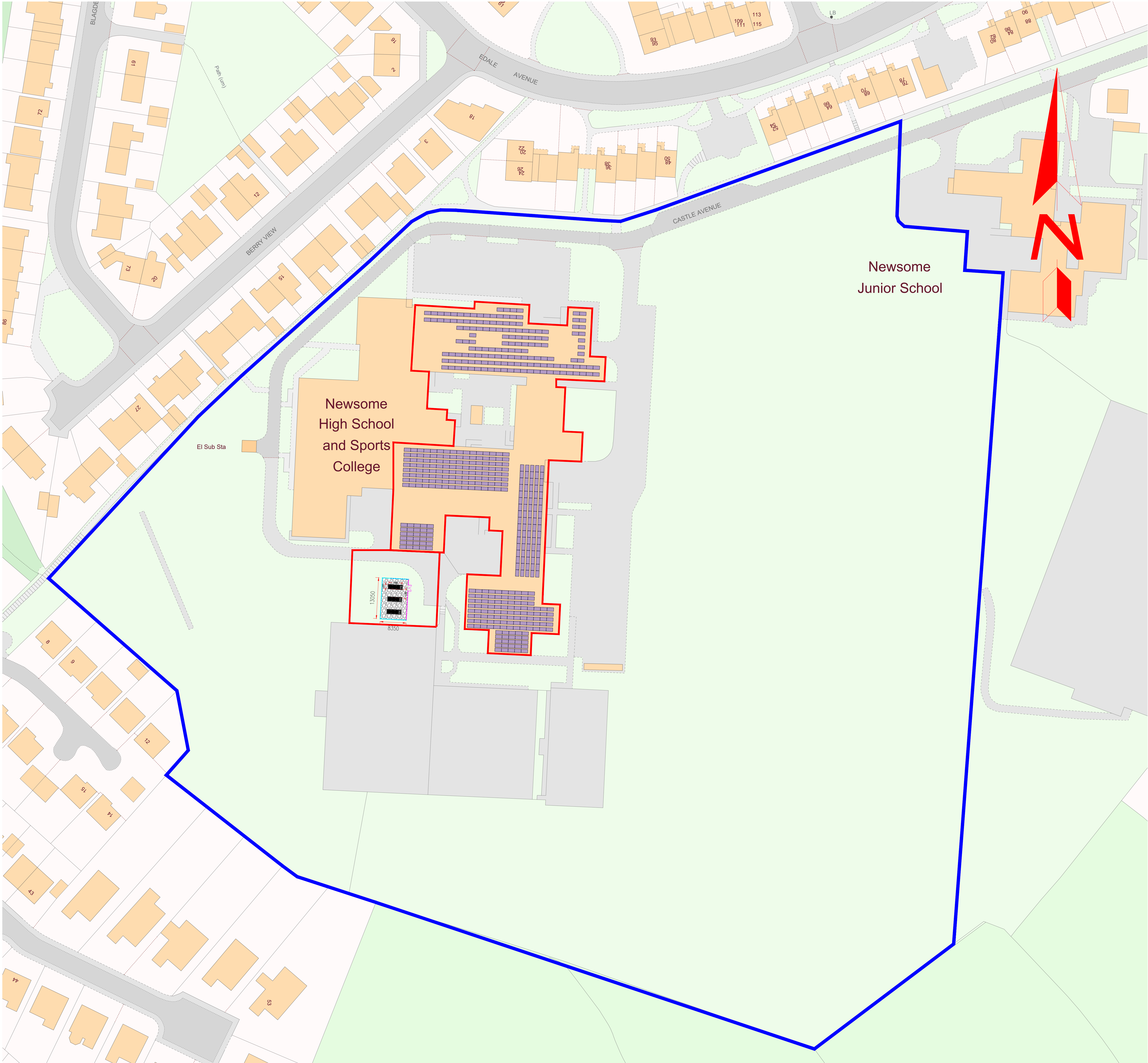
Site Block Plan - As Proposed 1:500
