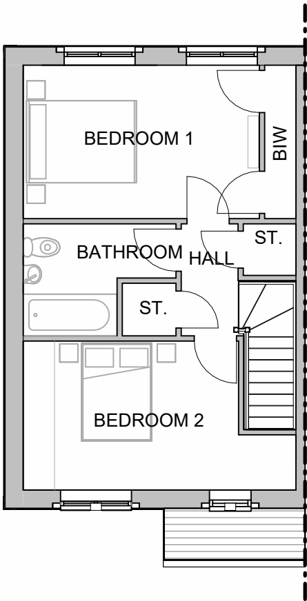
First Floor 1 : 100
