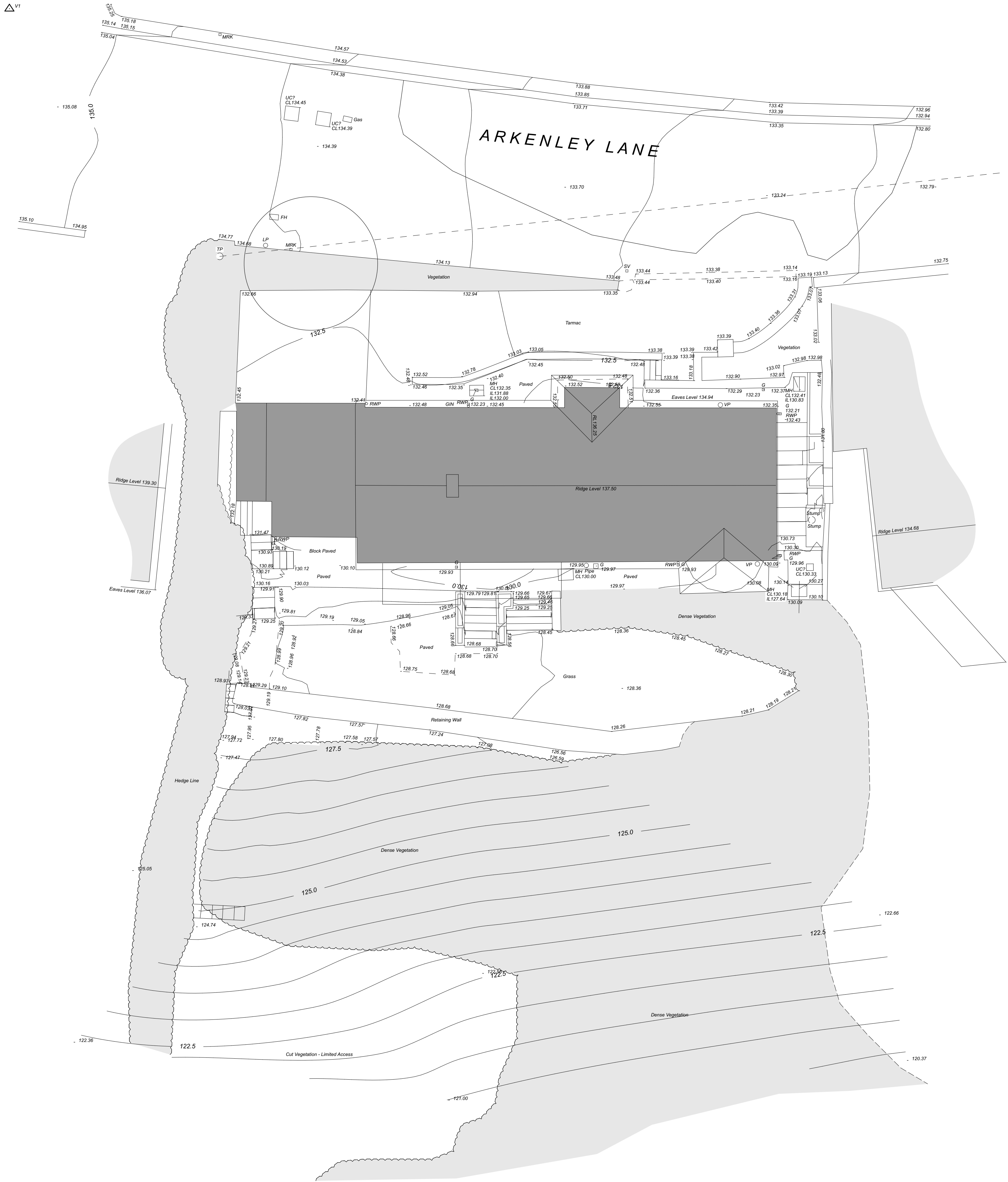
Topographical Survey - 1:100
