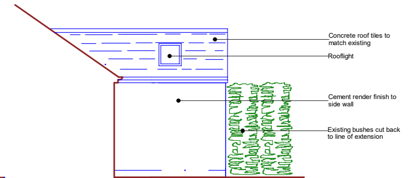
SIDE ELEVATION (South West)
