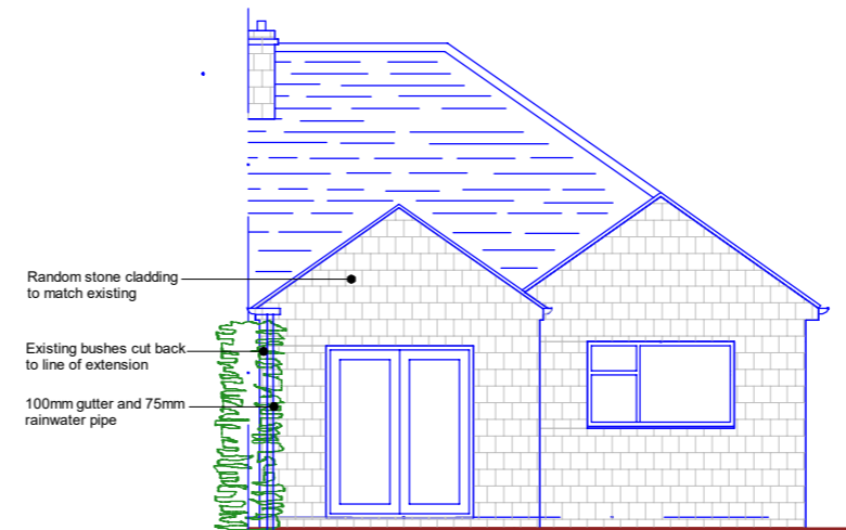
FRONT ELEVATION (South East)
