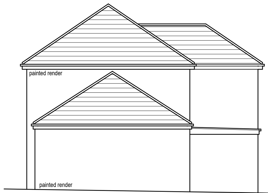
Proposed side/west facing elevation (1:100)
