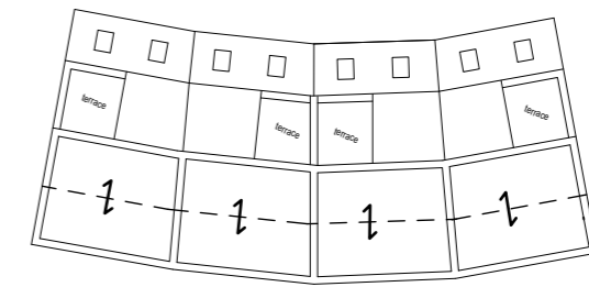
Roof layout (1:200)
