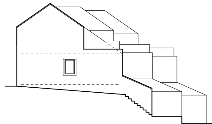
Side elevation (1:100)
