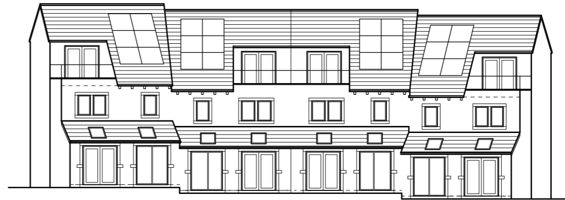
Rear/north facing elevation (1:100)
