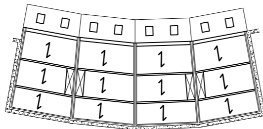
Ground floor TJI layout (1:200)
