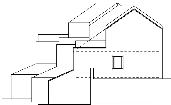
Side elevation (1:100)
