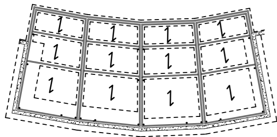
Foundation layout (1:200)
