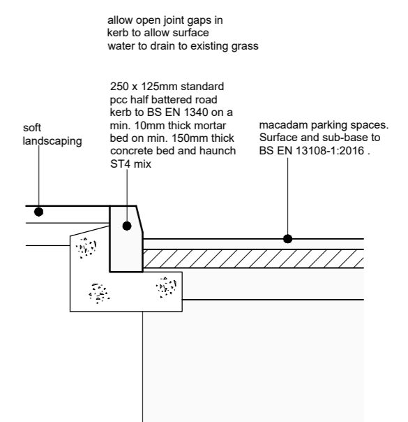
kerb detail
