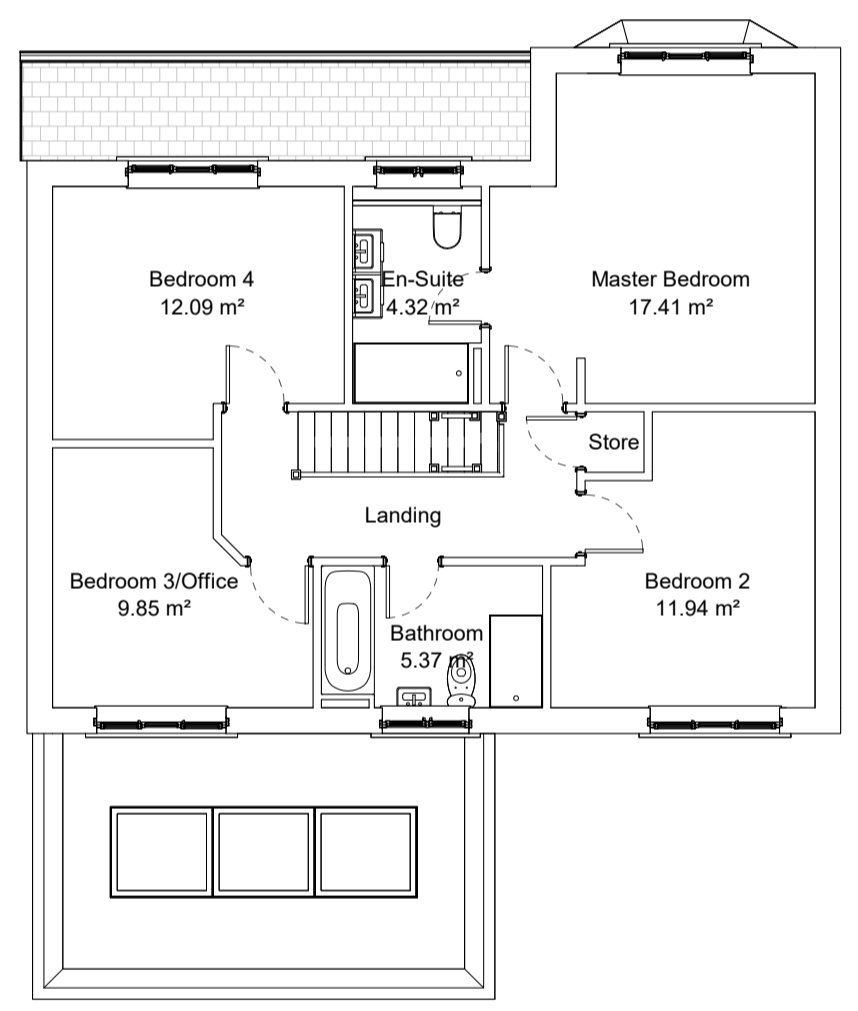
First Floor 1 : 100
