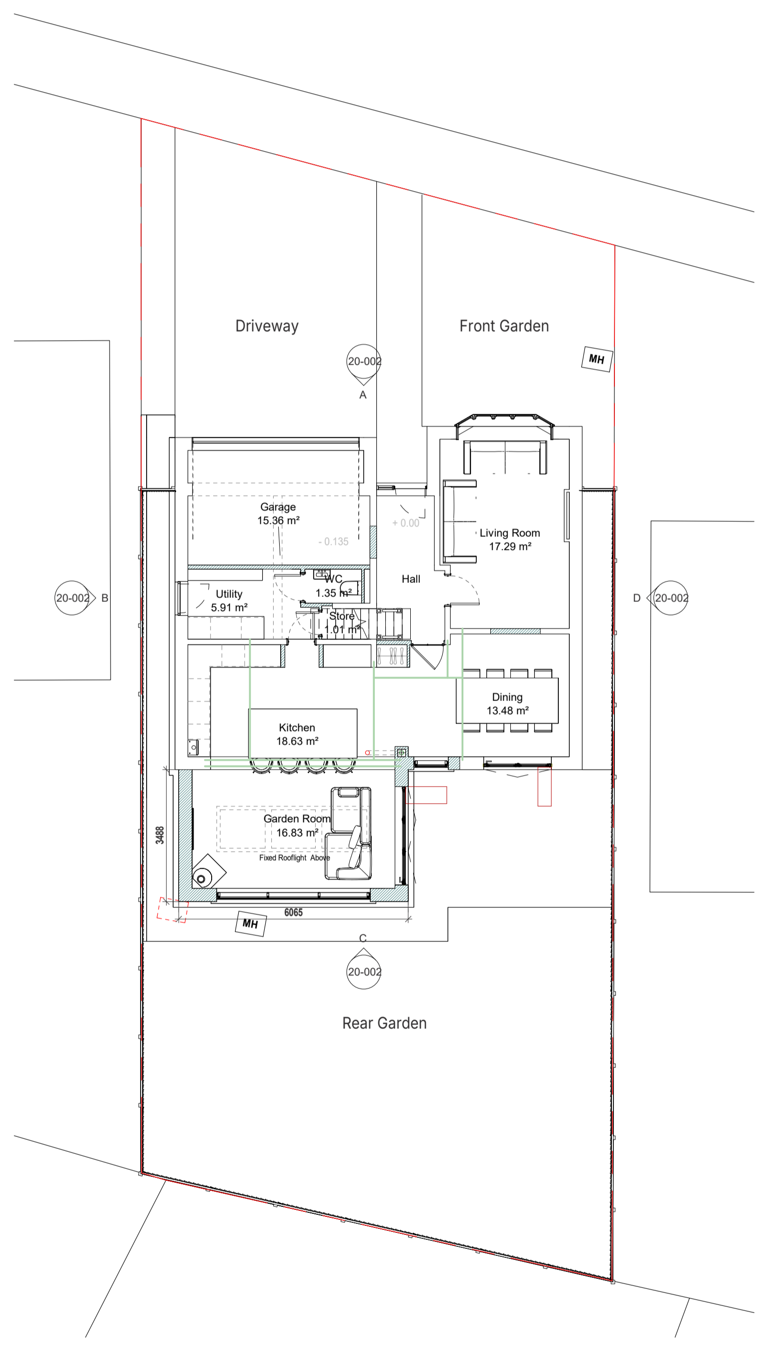
Ground Floor 1 : 100
