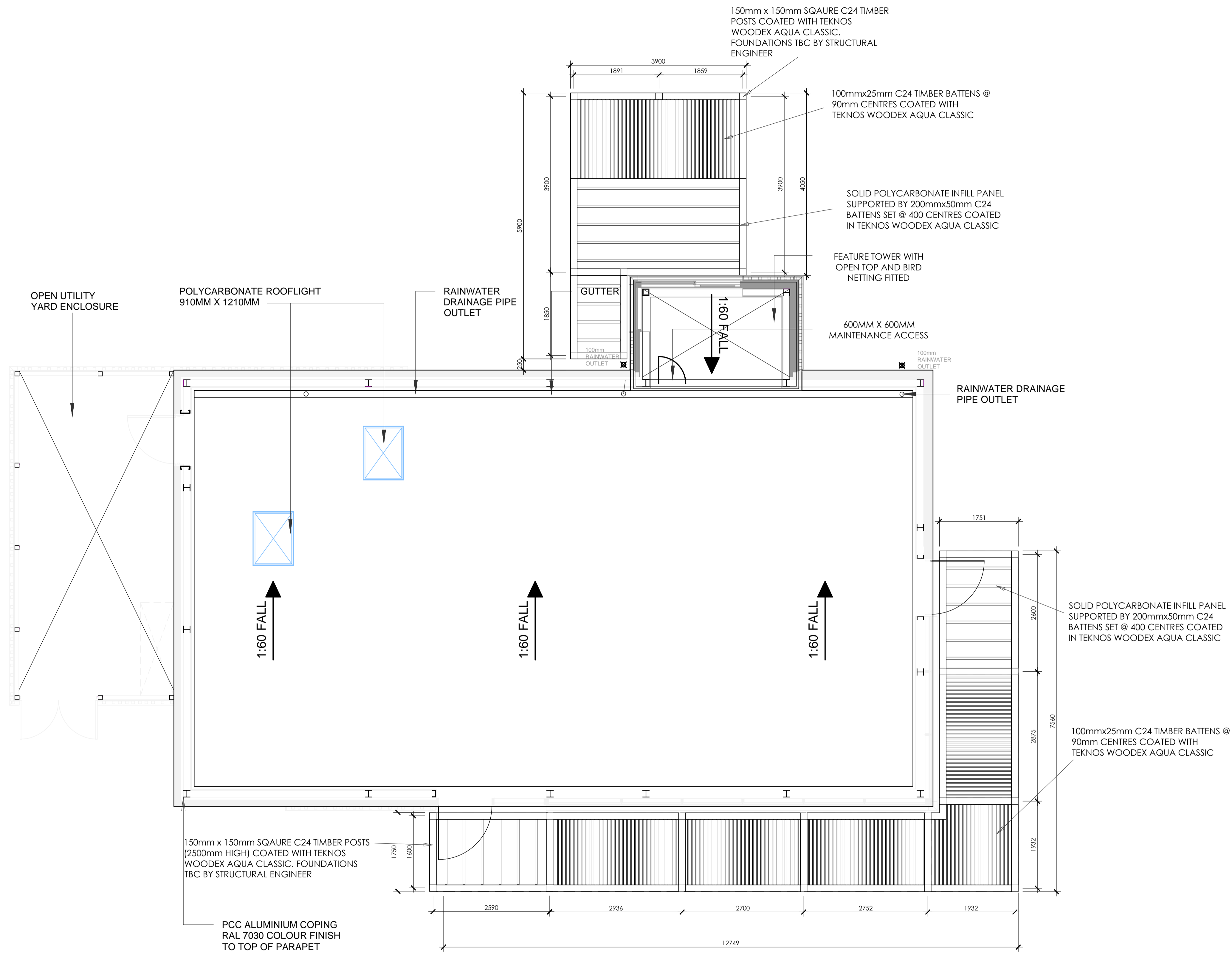
Proposed roof plan - scale 1:50 @ A1 / 1:100 @ A3
