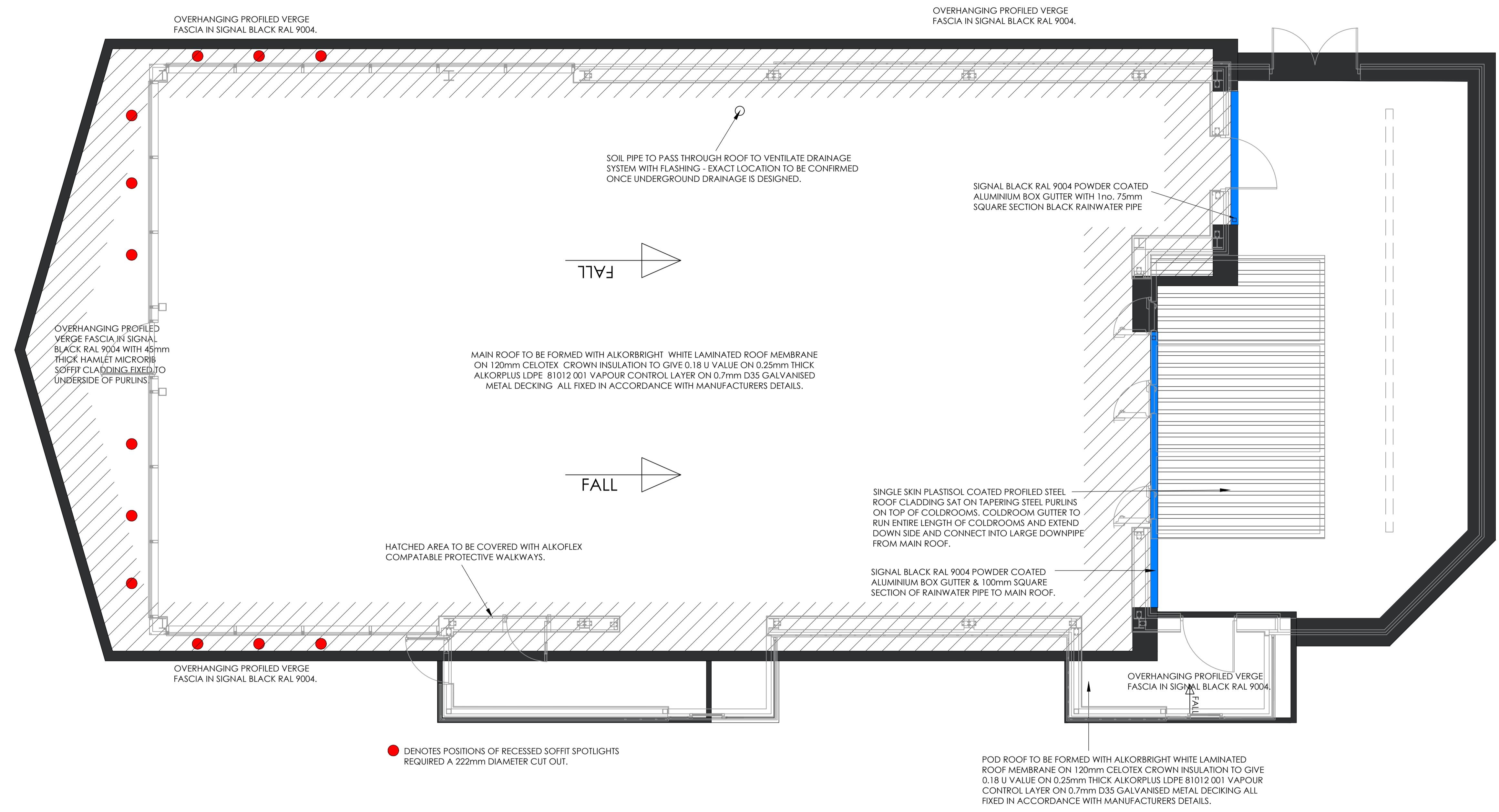
proposed roof plan - scale 1:50 @ A1 / 1:100 @ A3
