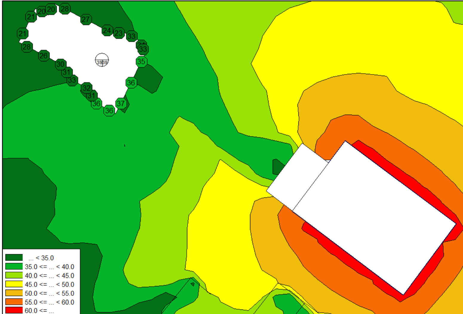
Figure D1: 1.5m high noise map - Daytime
