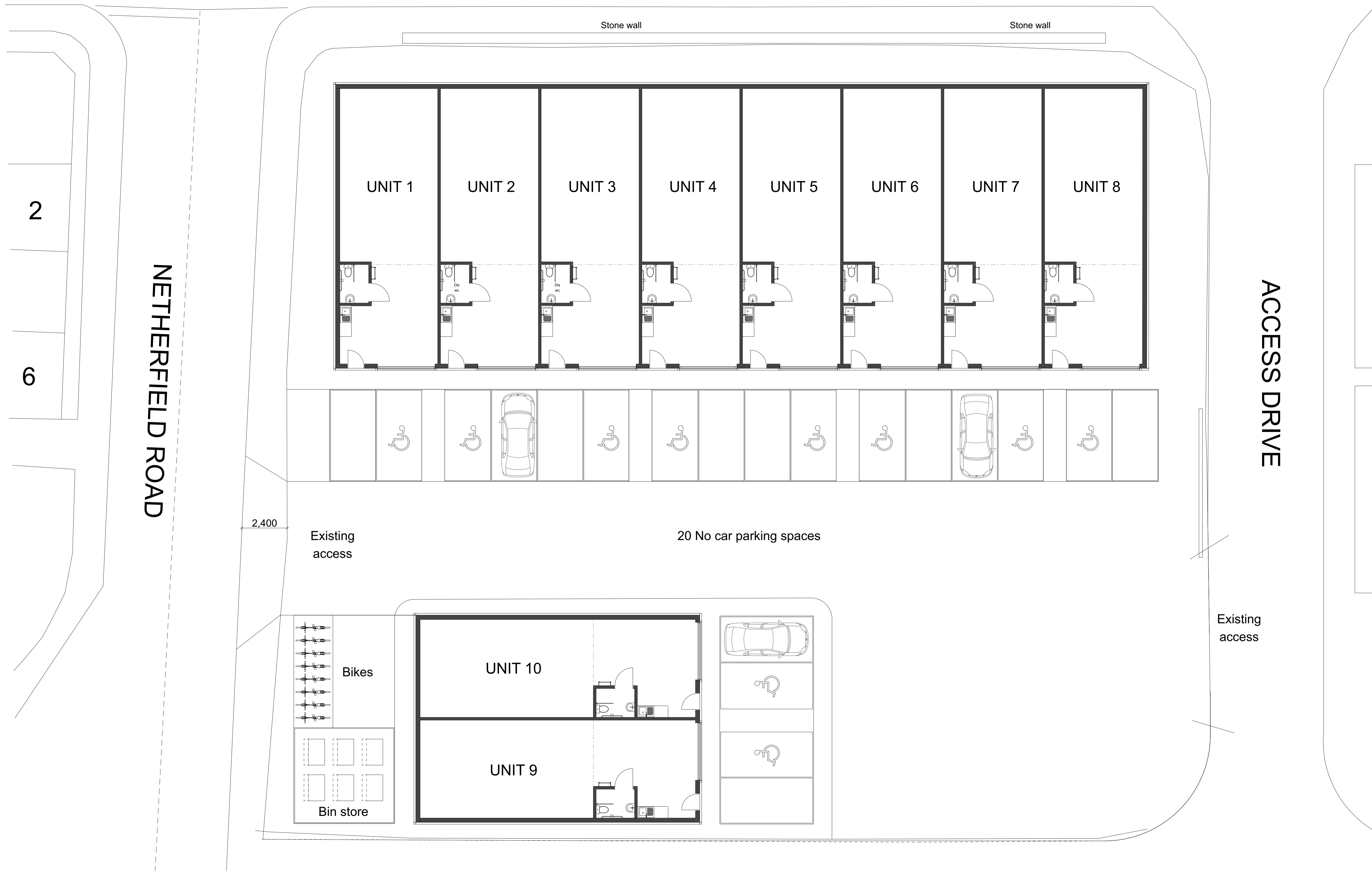
01 Proposed block plan Scale 1:100
