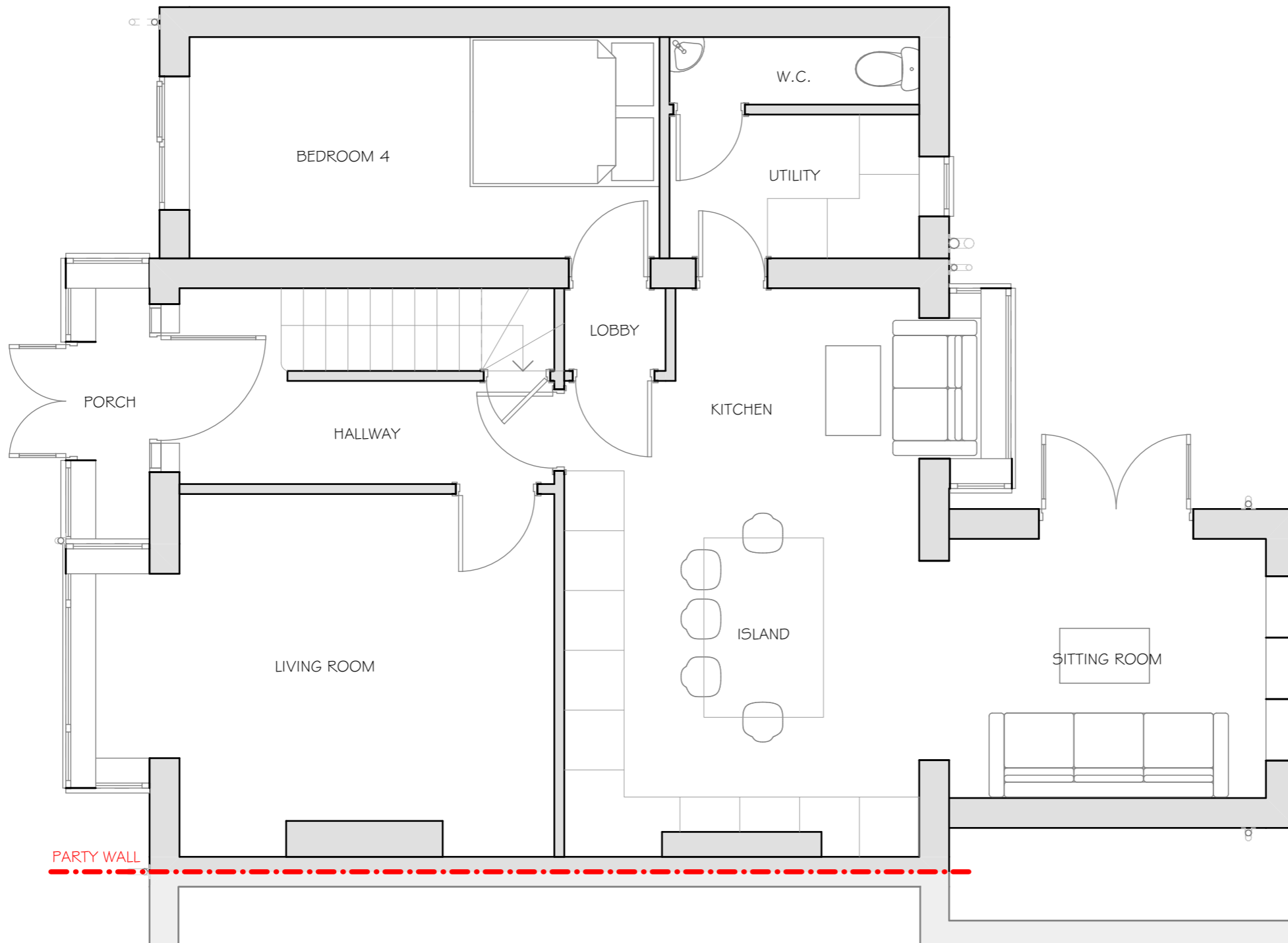
PROPOSED GROUND FLOOR PLAN 1:50@A3
