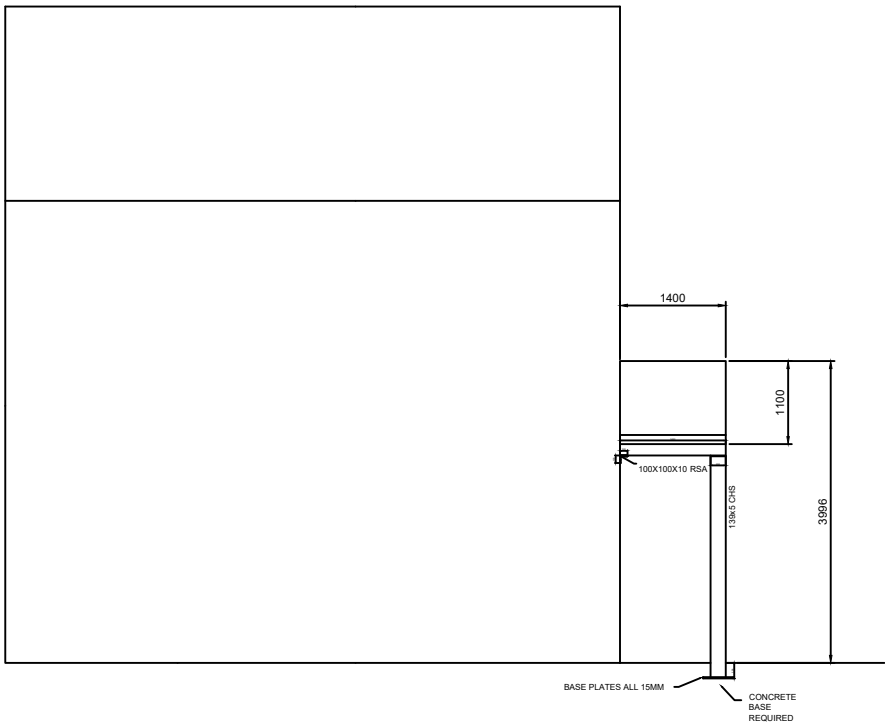
SIDE VIEW
