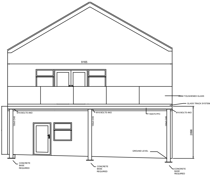
ELEVATION VIEW
