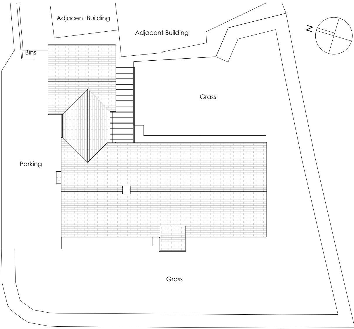
Block Plan 1:200
