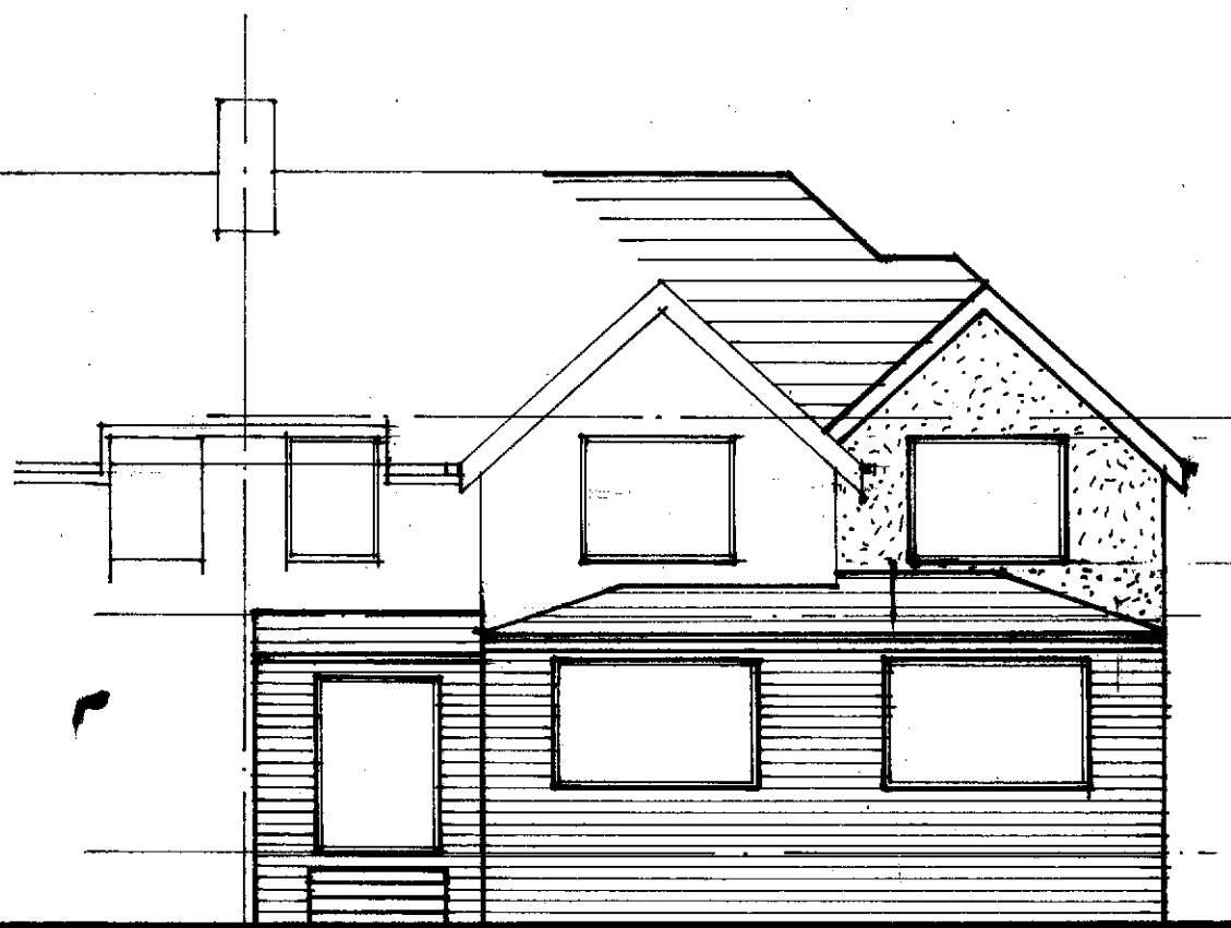
FRONT 1:100
