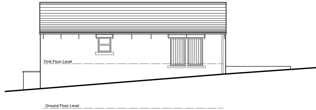
West Elevation (side)
