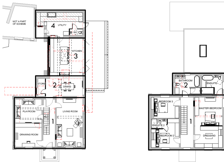
Floor plan proposed with corresponding building numbers. Ground Floor (Left) and First Floor (Right).
