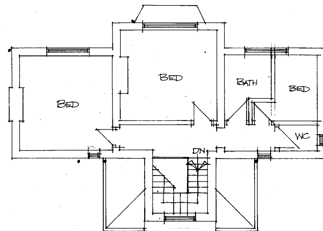
FIRST 1:100
