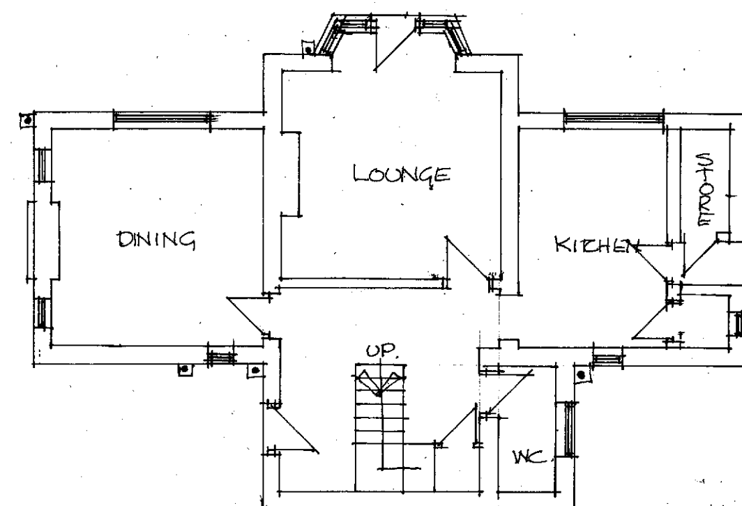
FRONT SIDE & REAR EXTENSIONS TO 12 CAWLEY LANE HECKMONDWIKE EX PLANS CLH/301
