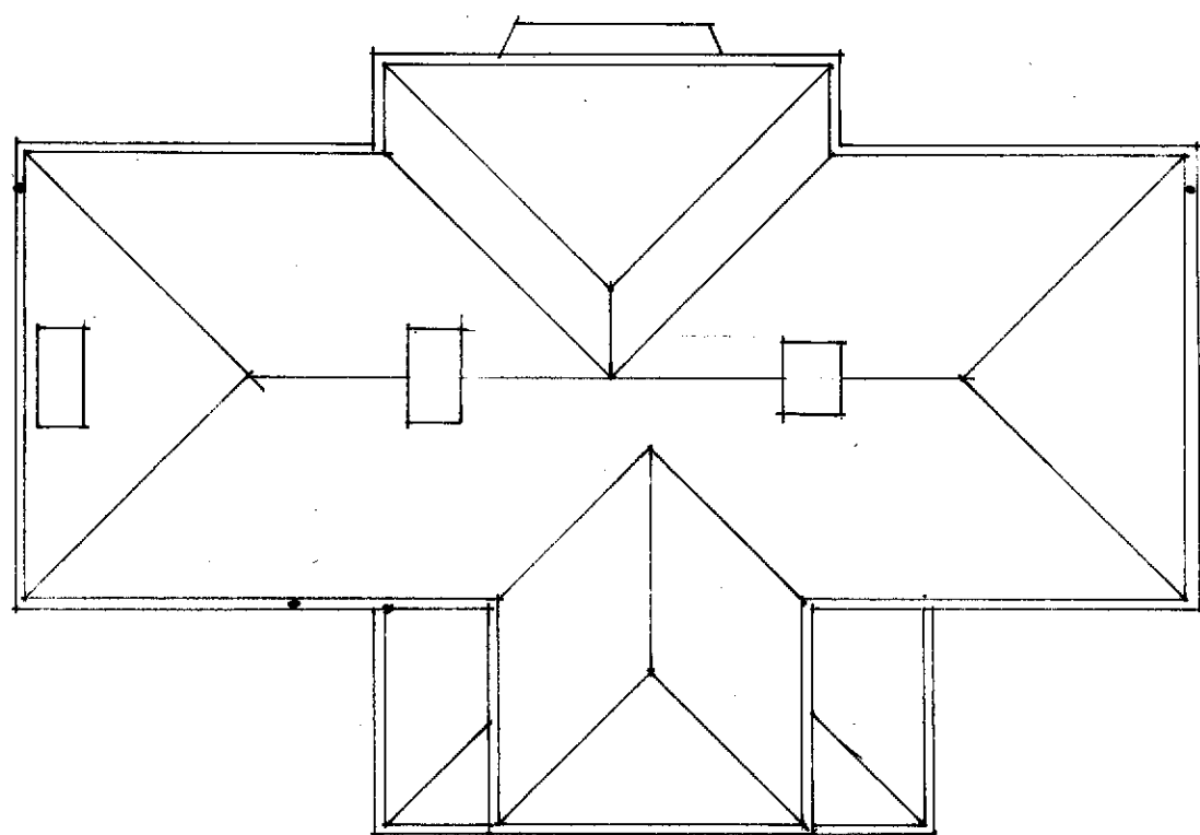
ROOF 1:100
