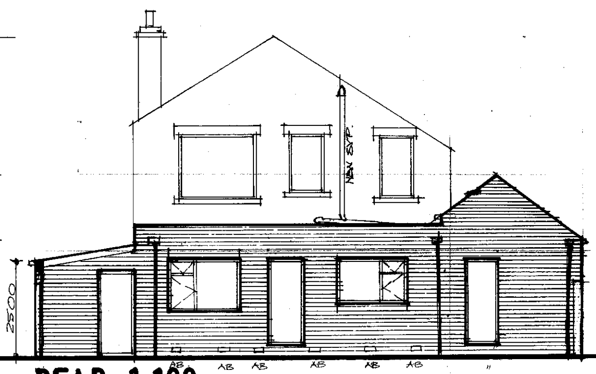
REAR 1:100
