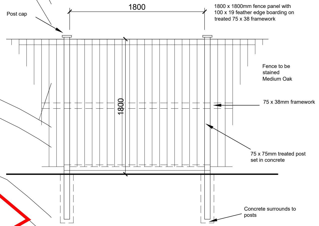
Fence Detail Scale at 1:25
