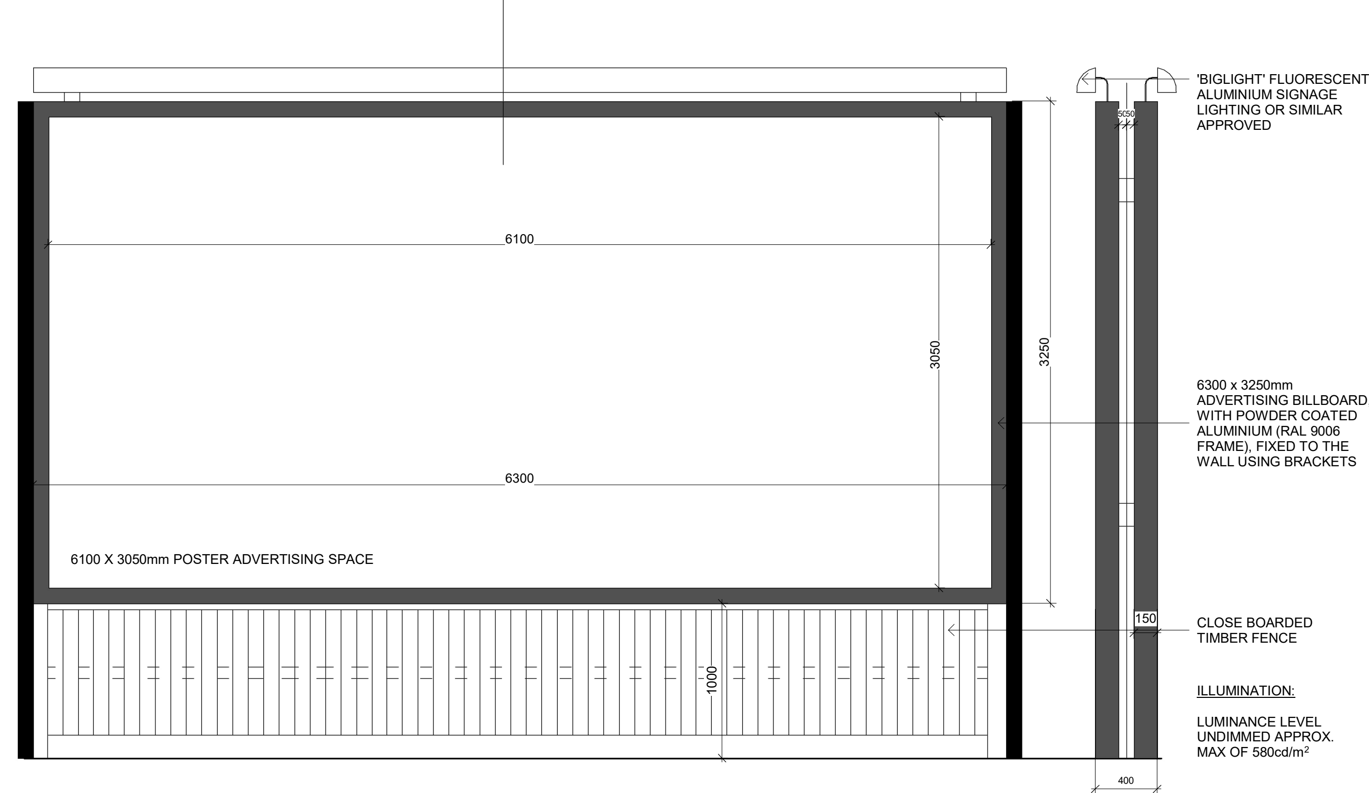
2 LARGE EXTERNAL BILLBOARD (1 No. TOTAL) 1:25
