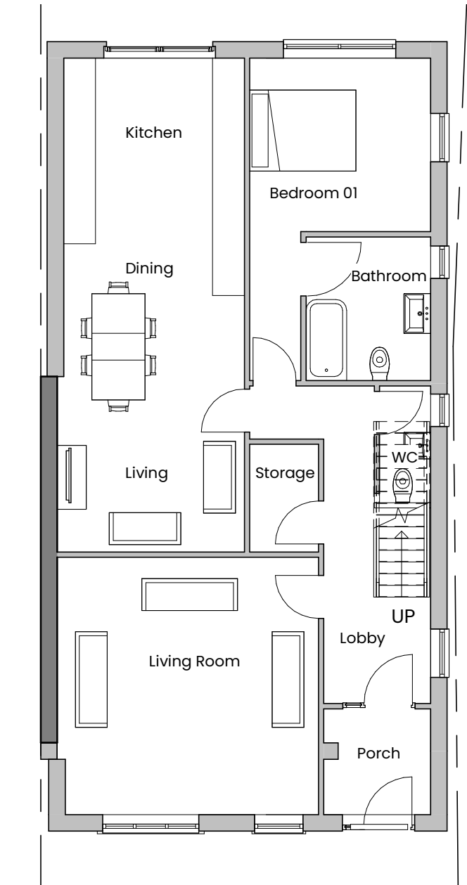
1 04. Proposed Ground Floor Plan 1:100
