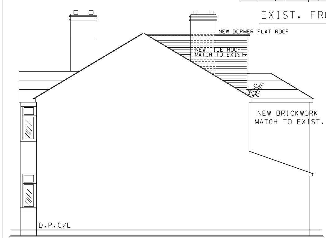
PROPOSED SIDE ELEVATION (VIEW 'Y')
