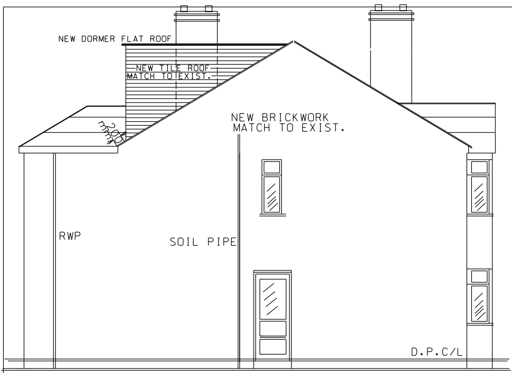
PROPOSED SIDE ELEVATION (VIEW 'X')
