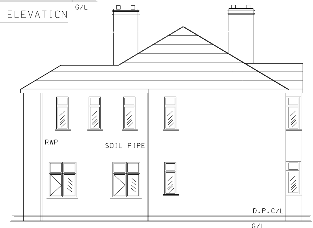
EXIST. SIDE ELEVATION (VIEW 'X')
