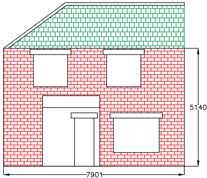
Front Elevation
