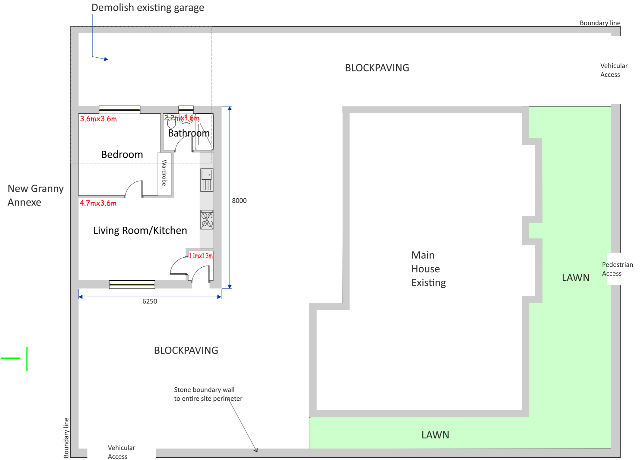
Proposed Site & Ground Floor Plan Scale 1:100
