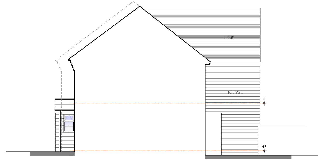
EXISTING WEST (SIDE) ELEVATION SCALE - 1:100
