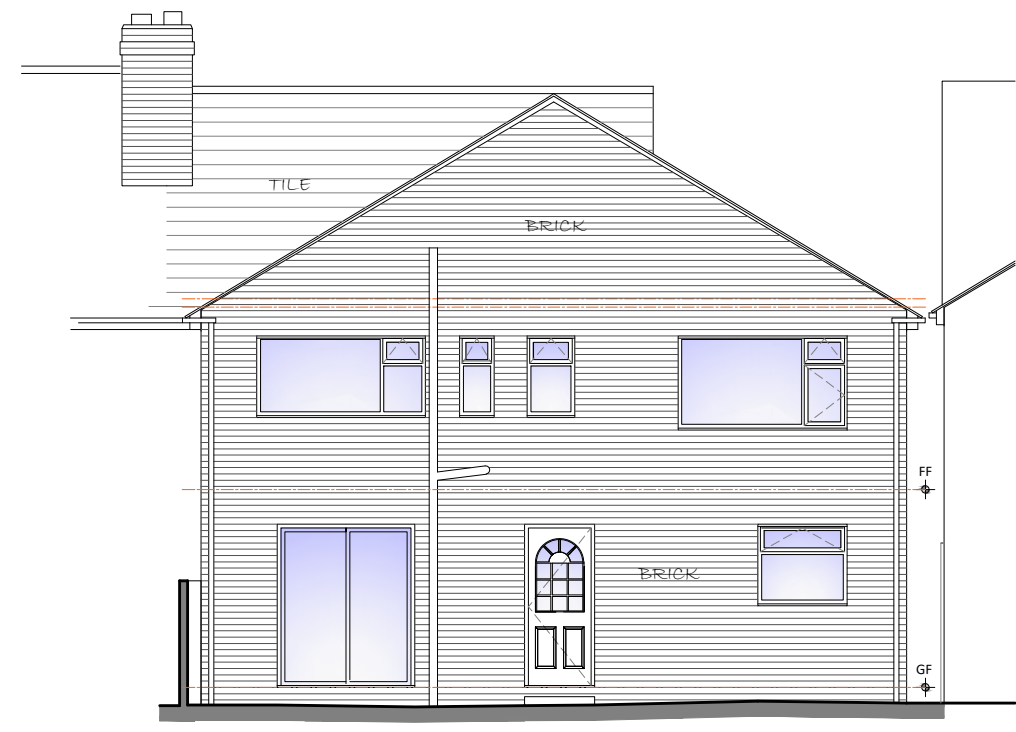
EXISTING SOUTH (REAR) ELEVATION SCALE - 1:100
