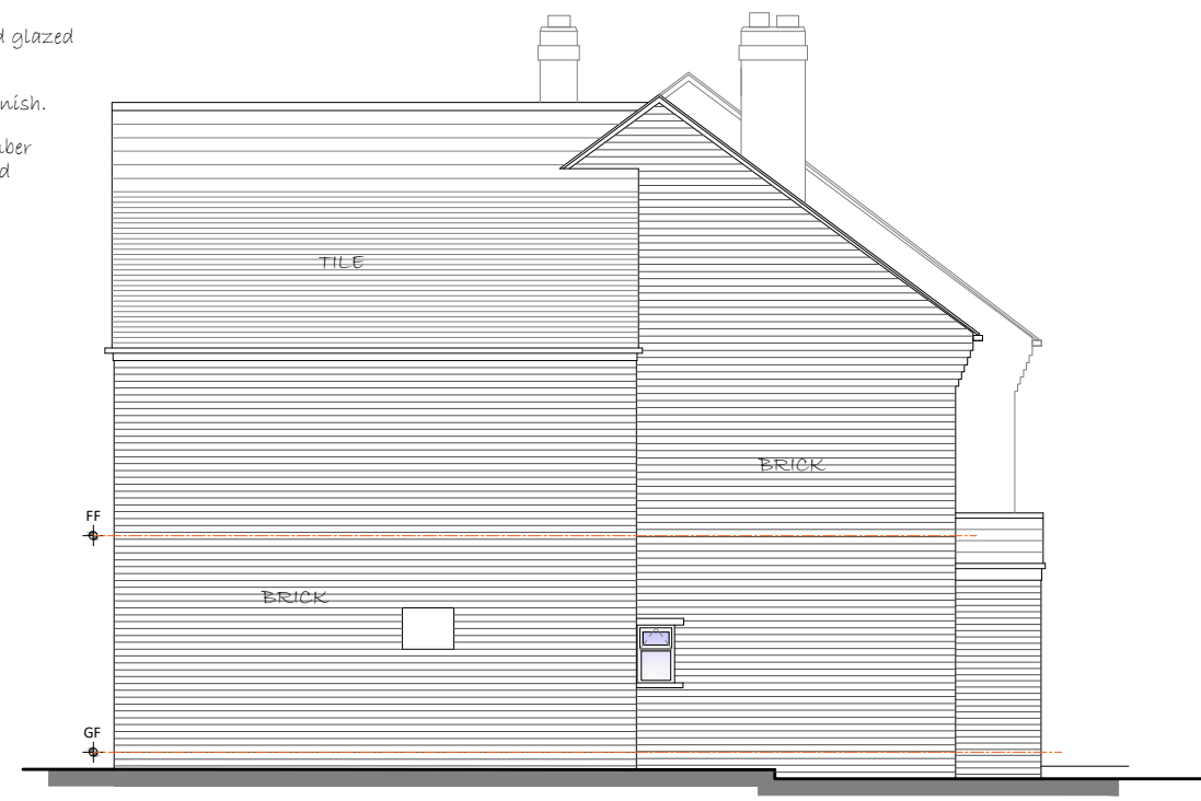
EXISTING EAST (SIDE) ELEVATION SCALE - 1:100
