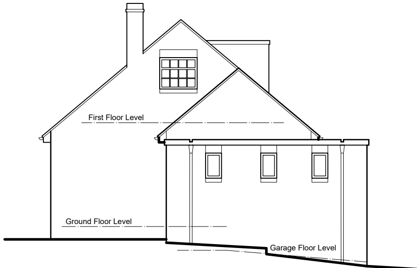
North east Elevation (side)
